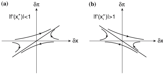
Fig. 1. We depict the orbits in the vicinity of the deterministic hyperbolic fixed point (x_1^*, 0) . In (a) we show the orbits in the case |f'(x_1^*)| < 1 , where the fixed point for the 1D map is stable. In (b) we show the orbits for |f'(x_1^*)| > 1 ; the fixed point for the 1D map is unstable.
