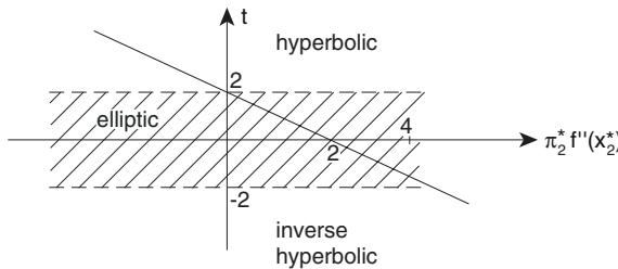
Fig. 4. We plot the trace t of the stability matrix M as a function \pi_2^* f''(x_2^*) . For t > 2 the fixed point is hyperbolic, for t < -2 the fixed point is inverse hyperbolic. For |t| < 2 the fixed point is elliptic.
