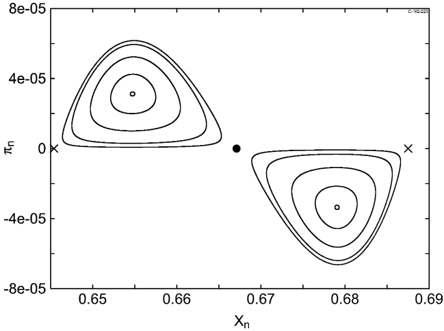
Fig. 5. The phase plane (x_n, \pi_n) for r = 3.004 just above the period-doubling into the two-cycle. The black dot is the now (hyperbolic) unstable fixed point; the crosses are the two-cycle on the x -axis and the KAM curves encircle the elliptic two-cycle.
