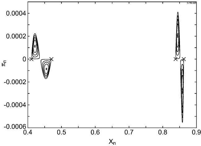
Fig. 7. The behaviour at r = 3.462 just above the period-doubling into the four-cycle. Note, the usual stable four-cycle on the axis and the associated elliptic four-cycle.
