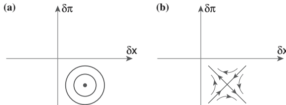
Fig. 3. We show the orbits in the vicinity of the noisy fixed point. In (a) we depict the elliptic case for |\pi_2^* f''(x_2^*) - 2| < 2 . In (b) we show the hyperbolic case for \pi_2^* f''(x_2^*) > 0 .
